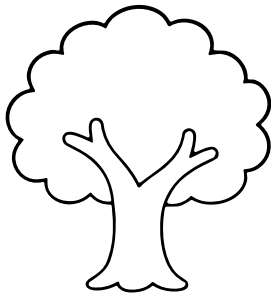
tree
