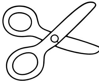
scissors
