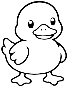
duck
