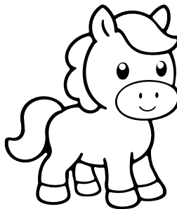
horse
