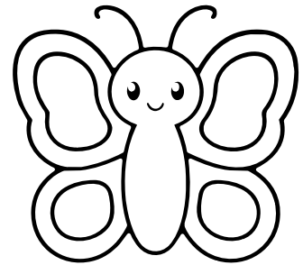
butterfly
