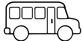
bus
